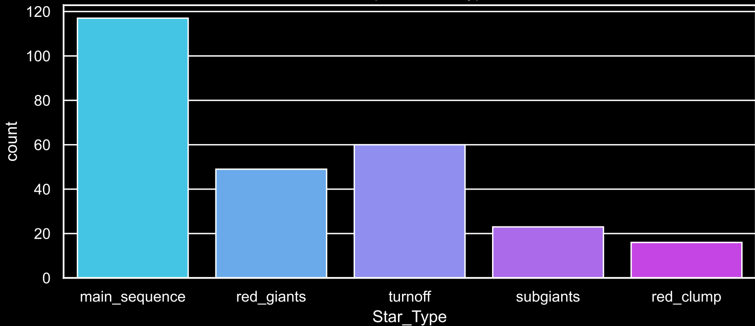
Field [68] Count plot of Star Type
