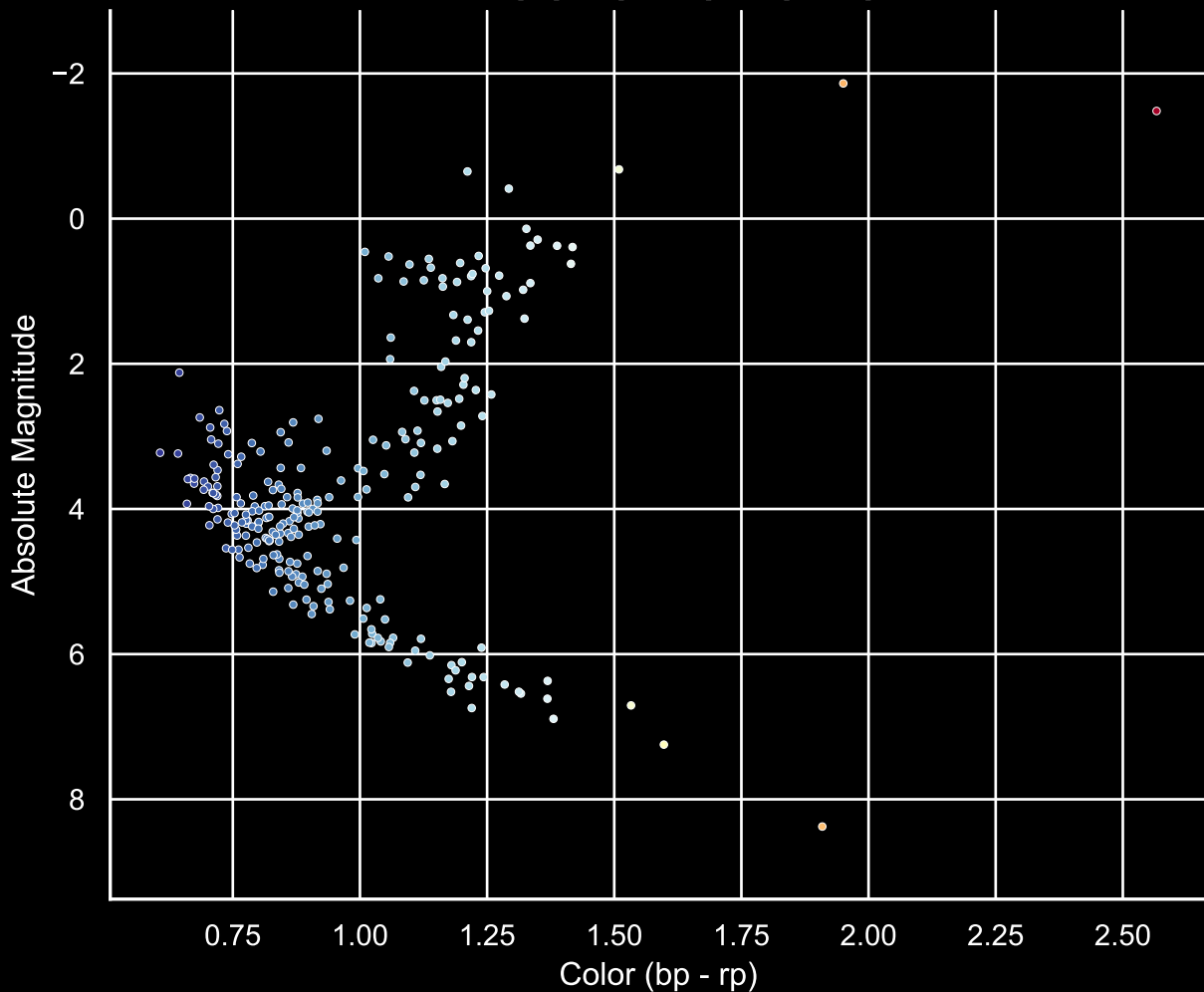
GALAH Hertzsprung-Russell Diagram Field [68] Ra [321.59] Dec [-23.43]
