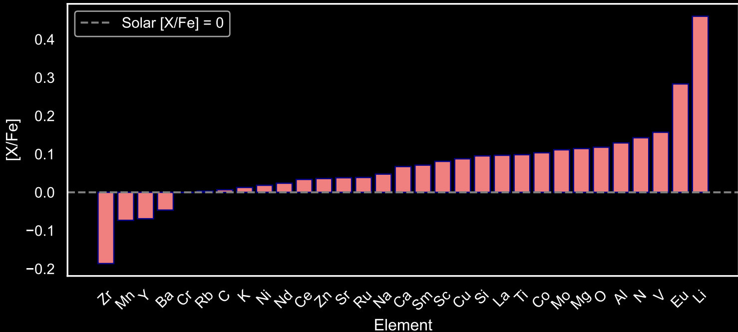
Abundance Pattern for GALAH Star Field [68] (N=265)
