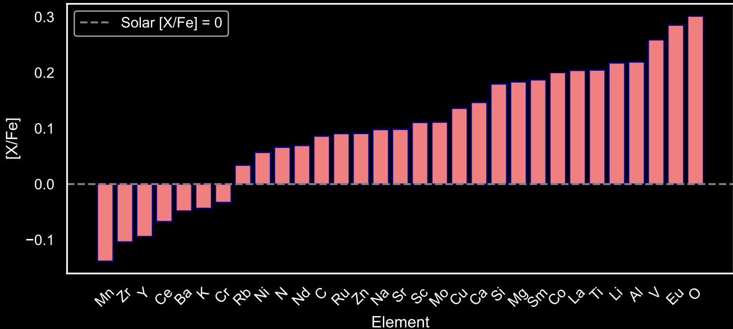
Abundance Pattern for GALAH Red Giants: Star Field [68] (N=65)
