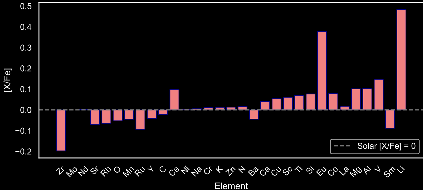
Abundance Pattern for GALAH Main Sequence Stars: Star Field [68] (N=117)
